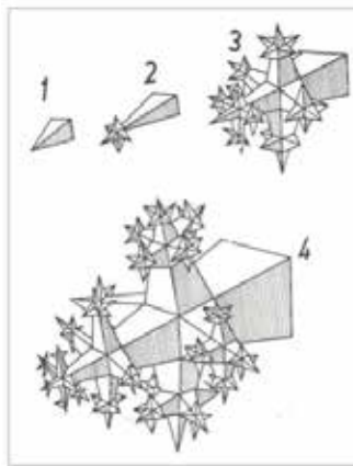
Fig 6: Dendritic growth from primary, secondary, tertiary to quaternary dimensions according to solidification time by Robert Wlodawer [7]
