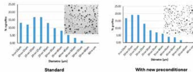
Figure 9: Comparison of graphite distribution between standard and new development.
