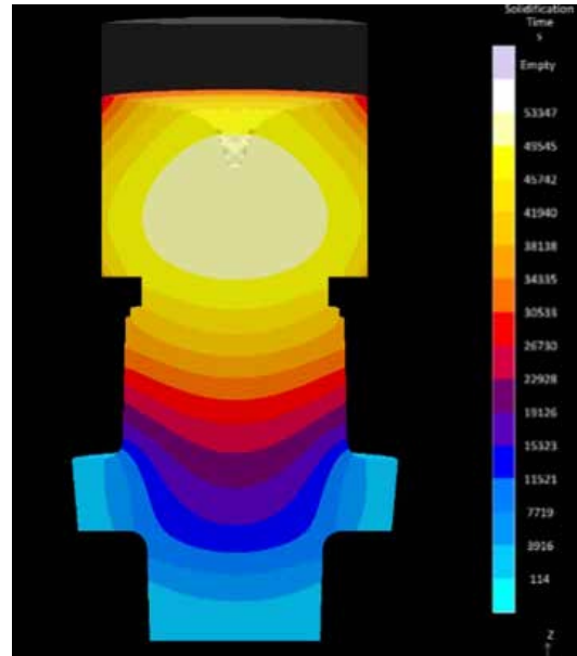
Fig 12b: Magma simulation of solidification time
