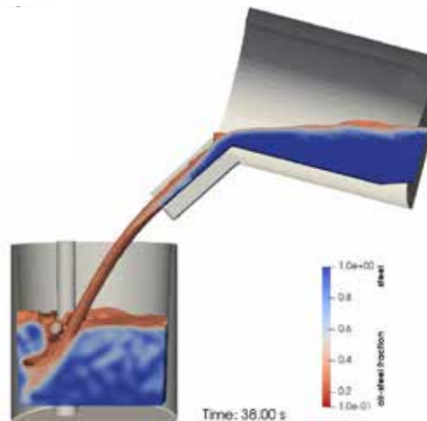
Fig 1b: CFD simulation of metal tapping
